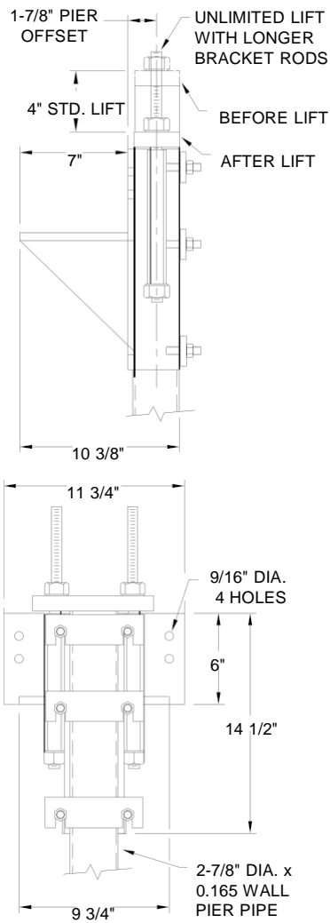
Model 300 Utility Bracket Details
