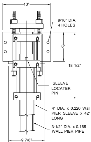
Model 350-EP2 - 2" Eccentric Utility Bracket Details
