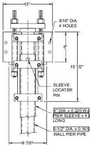
Model 350-MP2 Micro Pile Bracket Details
