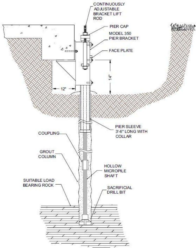
Model 350-MP2 – Typical Micro Pile Application Drawing
