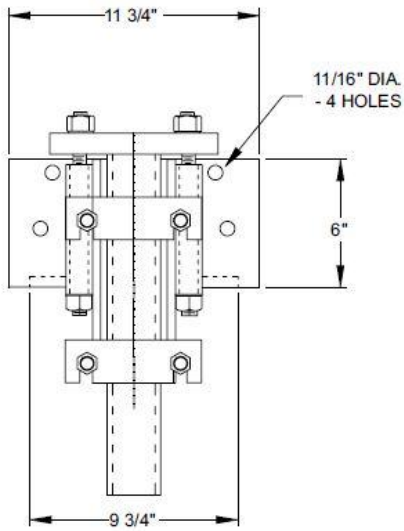
Model TAB-150-UB Utility Bracket Details
