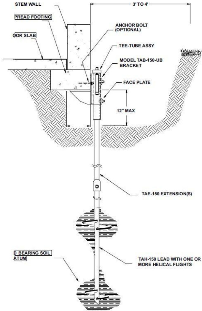
Model TAB-150-UB Utility Bracket Application Drawing
